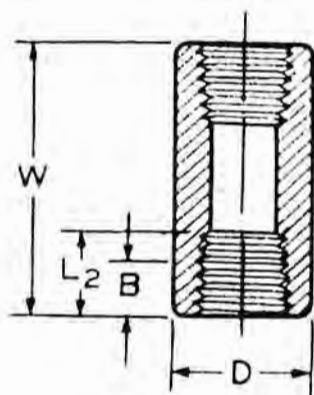
COUPLING
