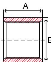
Fig. 29DC14 - 304 SS Recessed Drop Pipe Coupling
