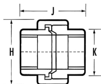
UNION
