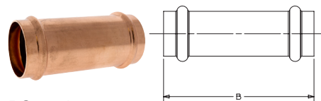
PC601L Extended Repair Coupling P x P
