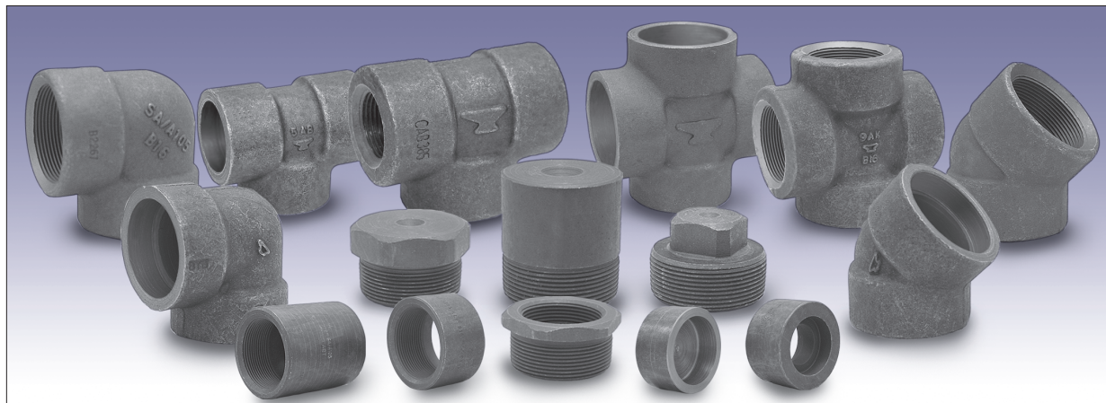
Fig. 2115 Crosses Fig. 2113 90° Street Elbows Fig. 2116 Laterals
