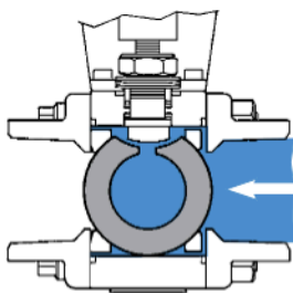
Valve shown in closed position, full pressure
