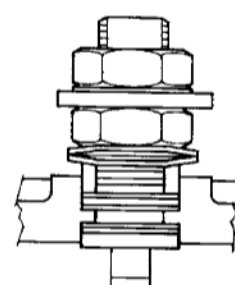
Manual Valve
