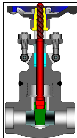
Welded Bonnet Design
